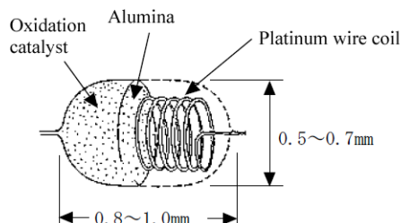
Structure diagram
