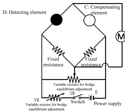
Basic circuit
